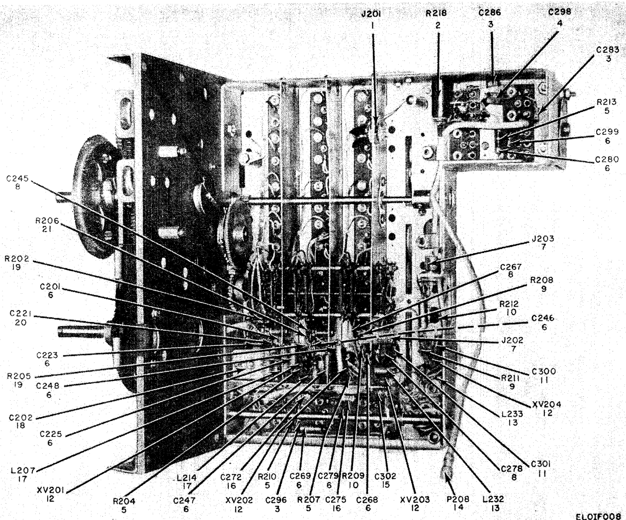
Figure 8. Amplifier, Radio Frequency, Full Bottom Interior View
